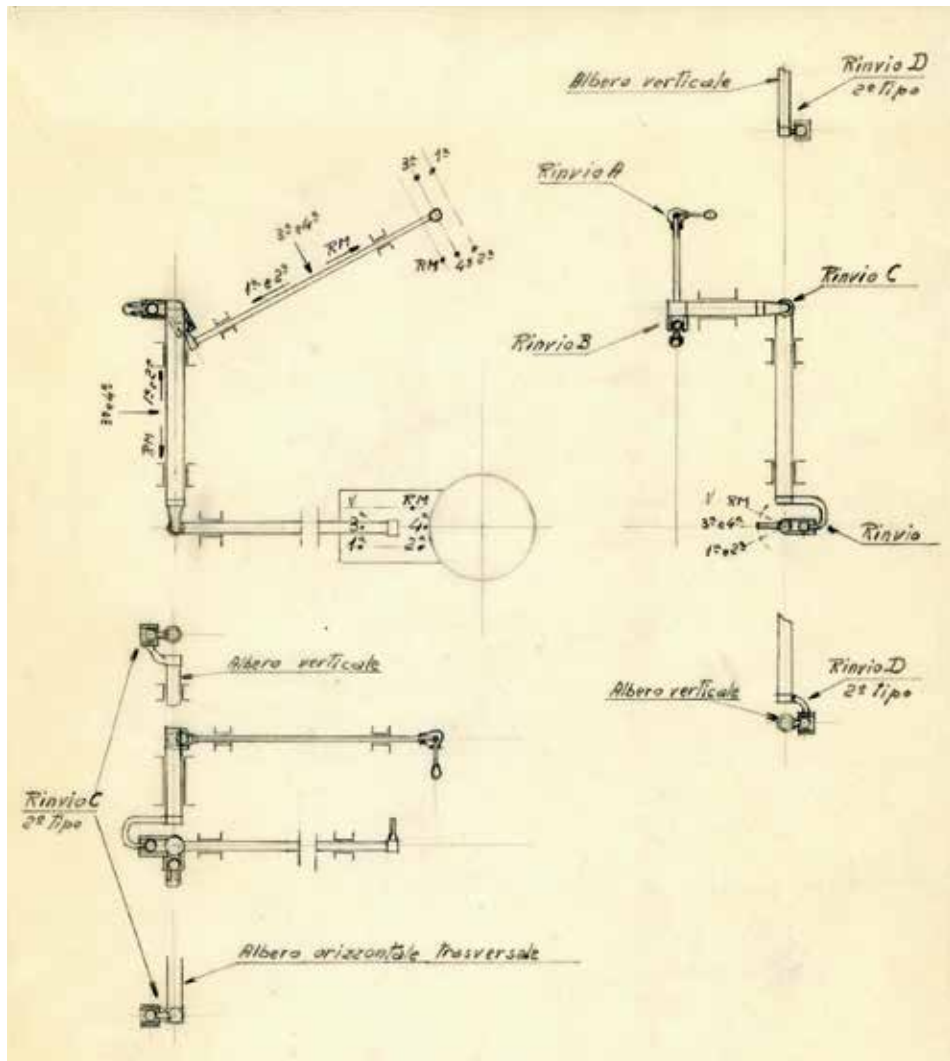
This sketch by De Virgilio in March 1947 outlined the gearshift linkage for the 50-degree car with its rear-mounted transmission. (De Virgilio Archive)
