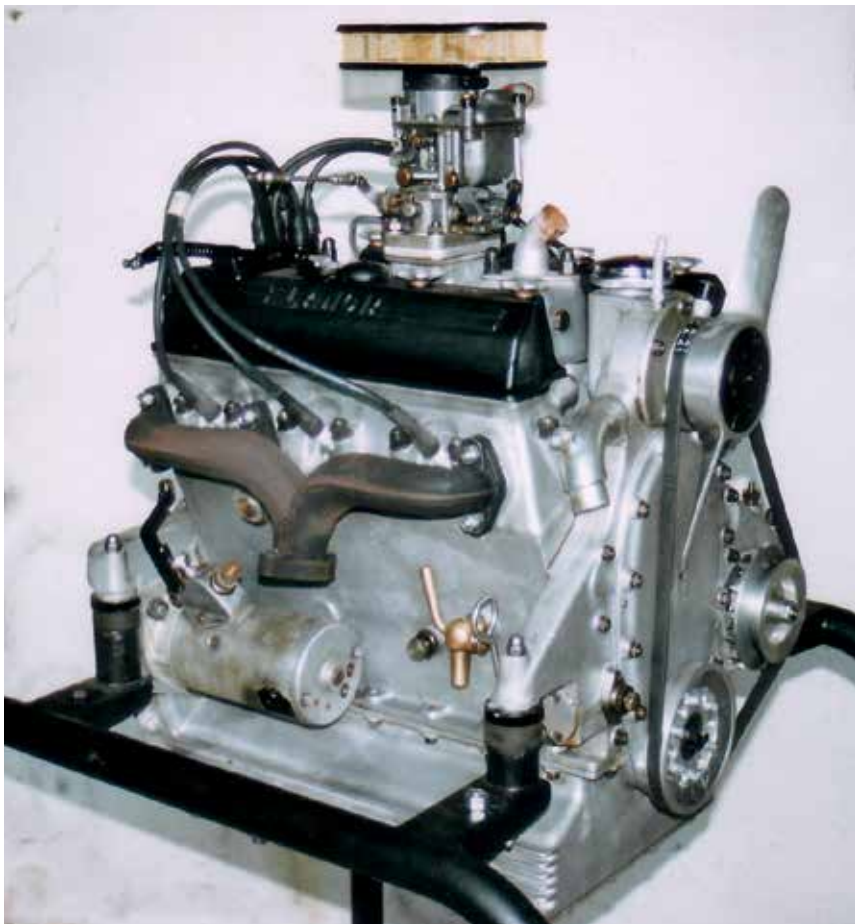
TOP The 538 motor was De Virgilio's first running V6. Two were made, including this one from 1946, recently restored. (Lancia Family Archive)
