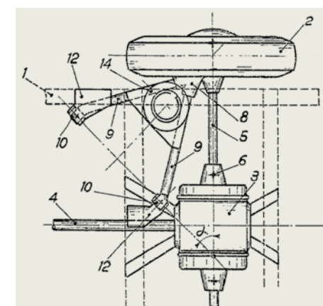
ABOVE LEFT AND RIGHT Lancia's 1947 patent drawings for the rear suspension show the semi-trailing arm (Nos. 9 and 14) but without offset bushings. The height of the pivot point (No. 11) was identified as an influence on the ride characteristics of the suspension, a subtle point not generally known at the time, now more widely appreciated. (Patent file No. IT 454511)
