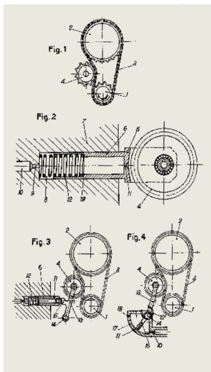
RIGHT Patent drawings for the hydraulic timing chain tensioner, from 1948. Fig. 2 shows hydraulic action on the the tensioning sprocket (4). Figs. 3 and 4 show alternate solutions not used. (Patent file No. CH 279415)
