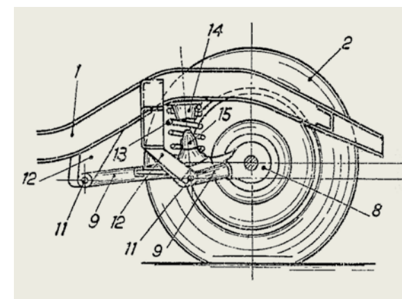
TOP The independent rear suspension of the Aurelia (for the right rear wheel). On the left of the drawing are the offset bushings for the semi-trailing arm; at the top of the drawing can be seen the outside universal joint located as far as possible from the inner pivot point, so as to reduce wear. (Automobile Engineer, 1951)
