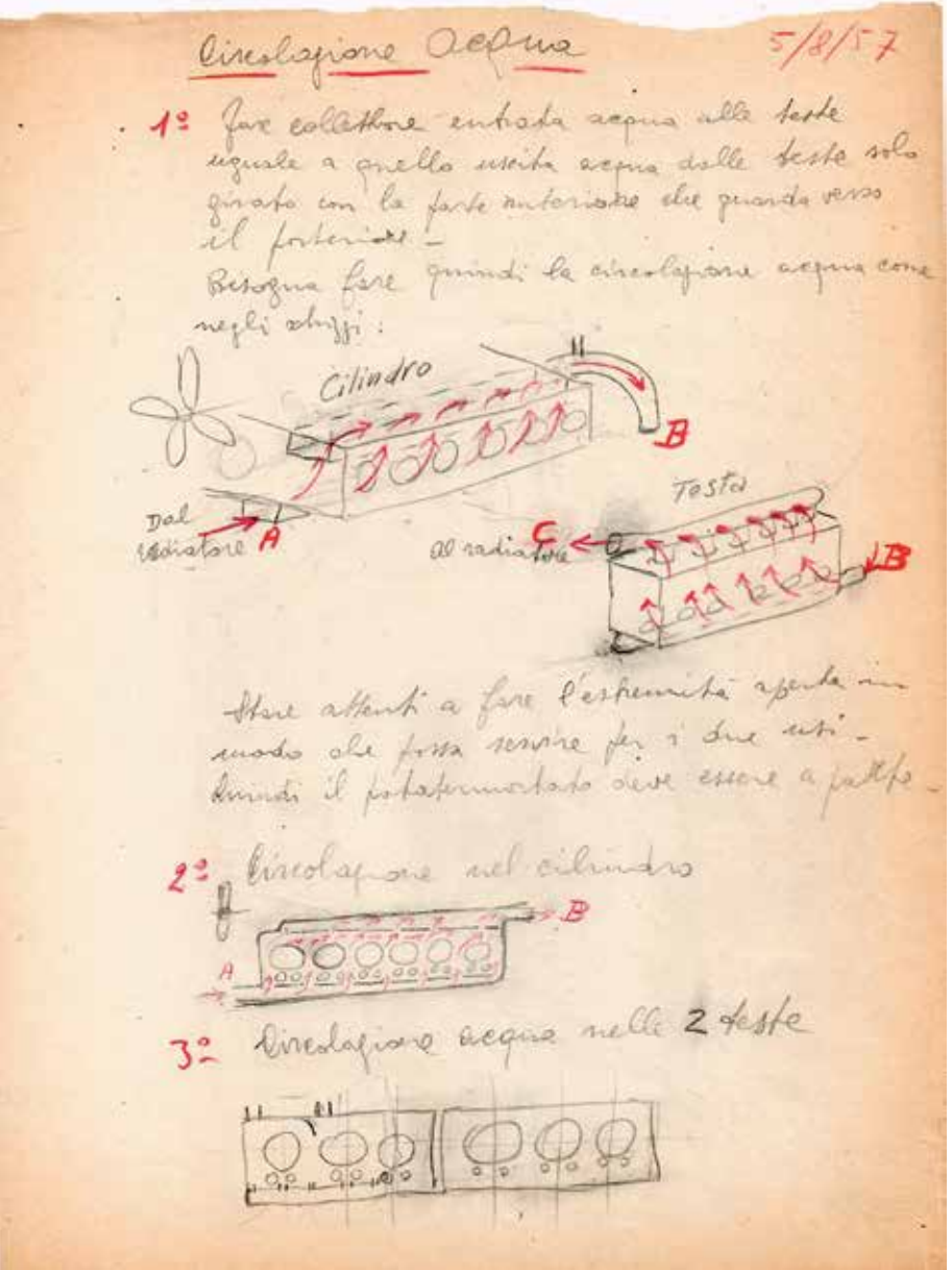
Preliminary sketch for the Esagamma, from 1957, analyzing water flow through the block and heads. (De Virgilio Archive)
